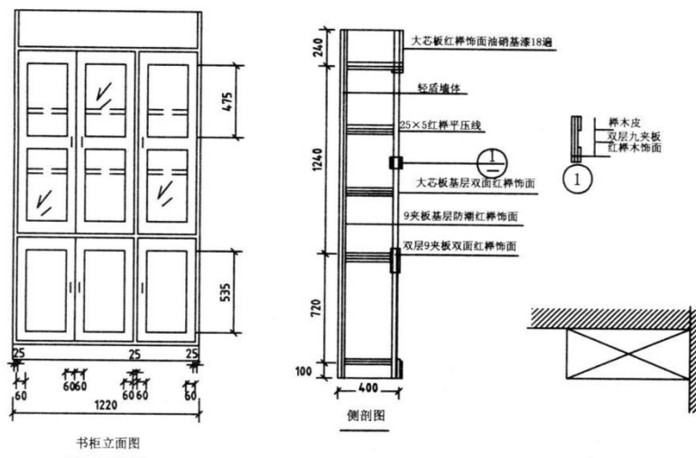
16-104 附墙书柜
